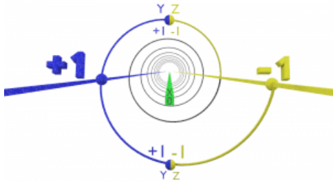
Illustration 9.8: Trinary Atom Waveform Full Size
