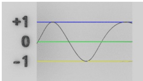
Illustration 2.2: 2D view of Trinary Logic
