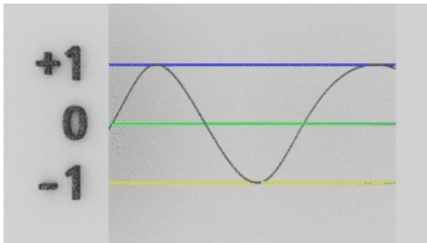
Illustration 5.1: Trinary Space Helix 2D Full Size
