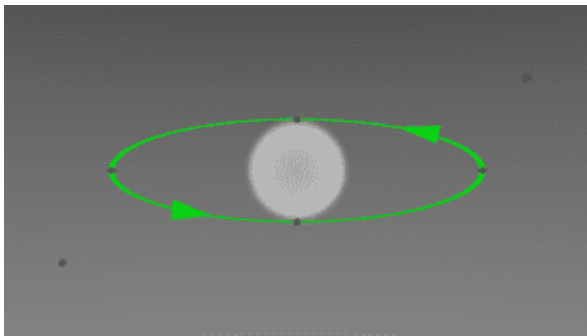
Illustration 9.13: Sun's Dark Stars Full Size
