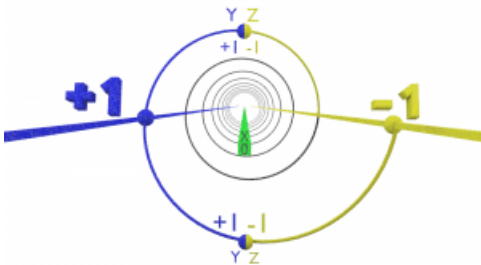
Illustration 5.2: Trinary Space Helix 3D Full Size
