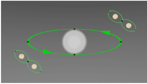
Illustration 9.15: One Arm Companion Dark Stars Full Size
