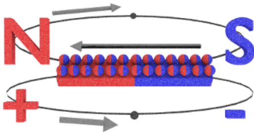
Illustration 7.3: Magnet with extra Electrons Full Size
