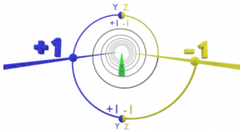
Illustration 9.7: Trinary Waveform Full Size
