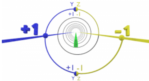
Illustration 2.1: 3D view of Trinary Logic
