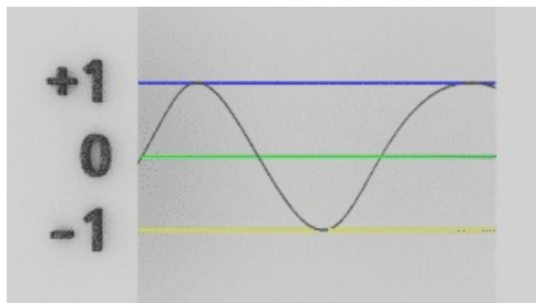
Illustration 9.9: Trinary Atom Waveform 2D Full Size
