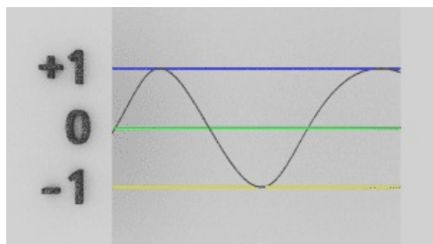
Illustration 9.10: Trinary Waveform in 2D Full Size
