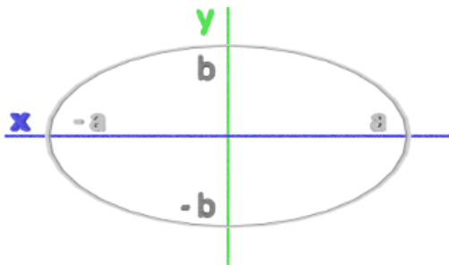
Illustration 7.6: Mathematical Graph of an Ellipse Full Size
