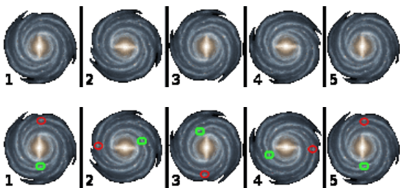
Illustration 9.16: The Galaxy Spinning all Solar Systems at the same Time Full Size Full Size
