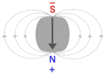
Illustration 7.1: Magnetic Poles of an Atom Full Size
