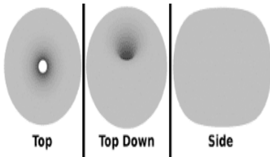
Illustration 9.2: Trinary Universe Sphere Full Size
