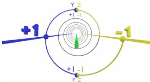
Illustration 7.4: An Electron Orbital Path around a Magnet Full Size
