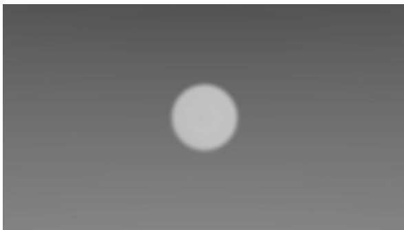
Illustration 9.11: First Stage of a Galaxy Full Size
