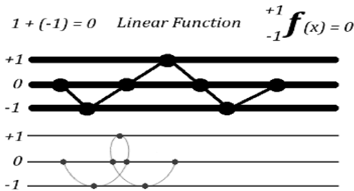
Illustration 9.3: Trinary Mathematical Formula Full Size
