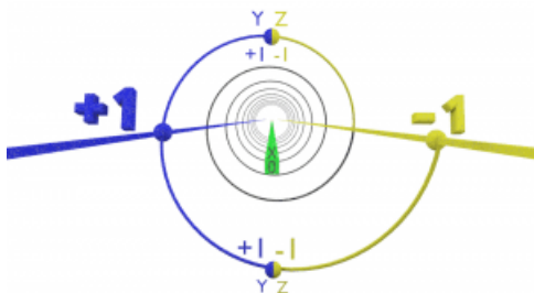
Illustration 9.6: Trinary Helix Full Size
