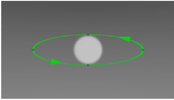
Illustration 9.12: Galaxy's Dark Stars
